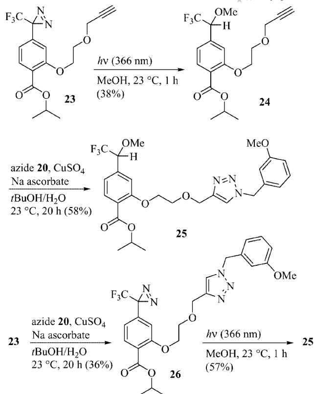
Scheme 4. Photoreaction of the alkynyl-functionalized phenyl(trifluoromethyl)diazirine 23 in methanol followed by a click reaction with benzyl azide 20 .
