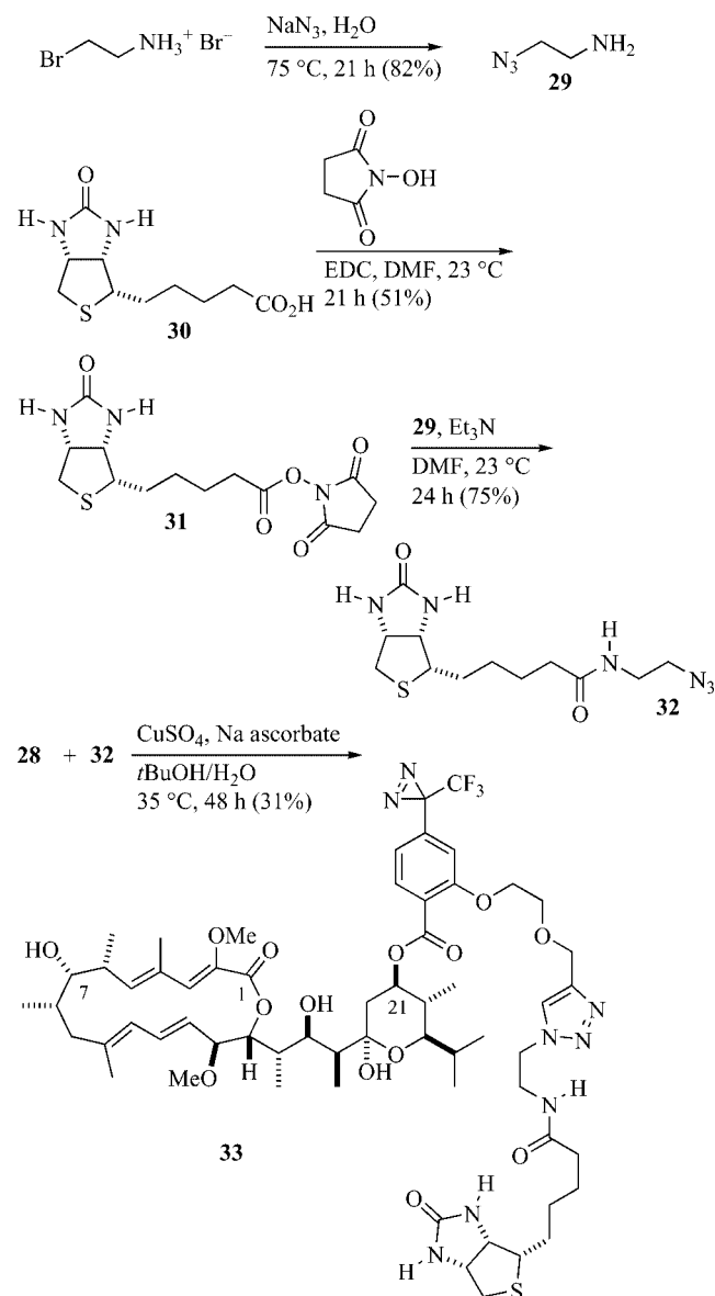
Scheme 6. Synthesis of the biotin azide 32 and its click reaction with the alkyne 28 .
