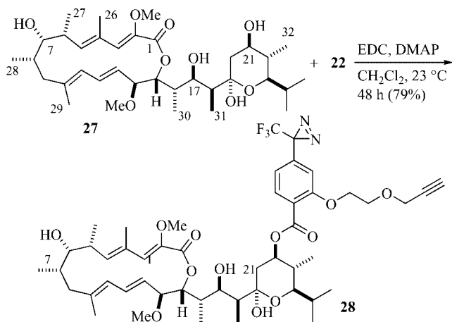
Scheme 5. Esterification of bafilomycin A 1 ( 27 ) at 21-OH with acid 22 yielding ester 28 .
