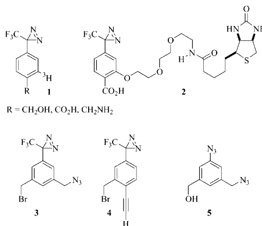
Figure 1. Some important examples of photoaffinity probes based on 3-(trifluoromethyl)-3 H -diazirines and azides.
