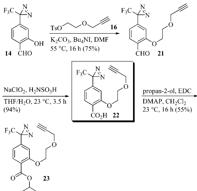
Scheme 3. Synthesis of the photoaffinity probe 22 by alkylation of phenol 14 and oxidation of the benzaldehyde 21 .
