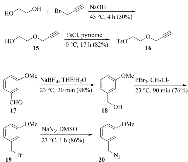
Scheme 2. Preparation of the alkyne 16 and benzyl azide 20 .
